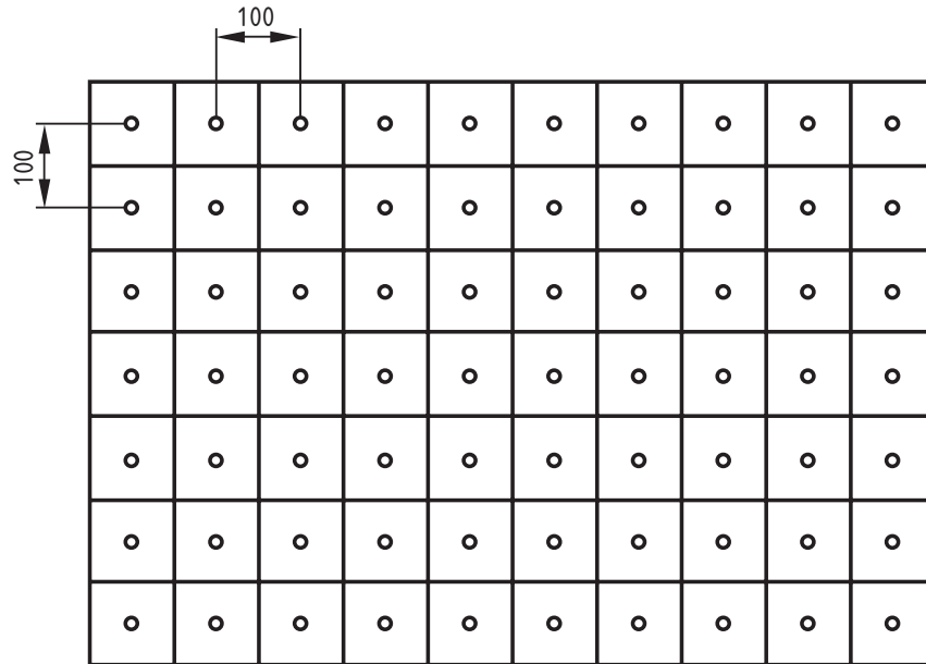
Figure A.6 — Plan view of trihedron hearth and walls showing position of possible measurement points
